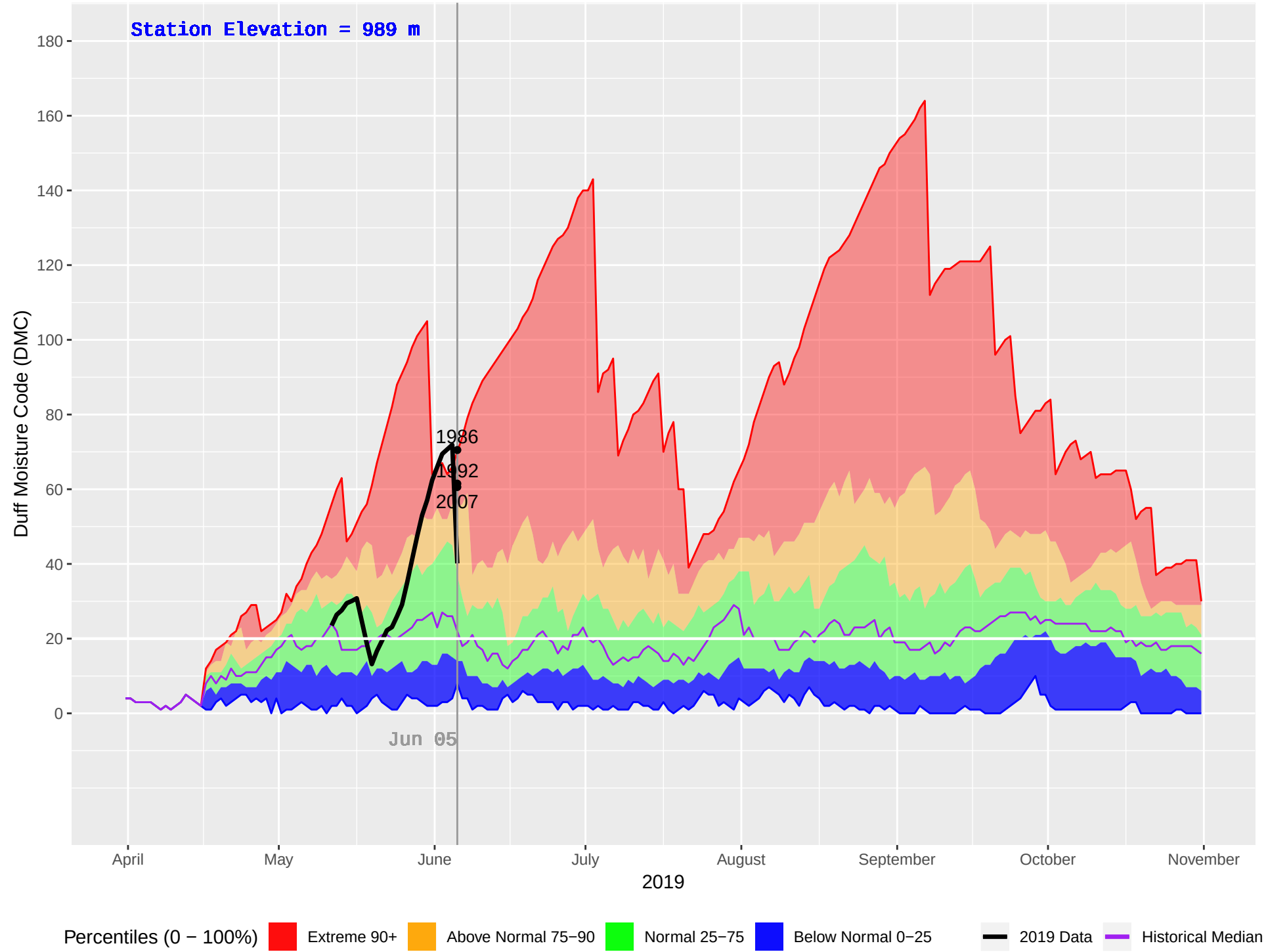
PINK MOUNTAIN (129) : Historical (1983–2018), Current (2019) Daily Duff Moisture Code (DMC)
