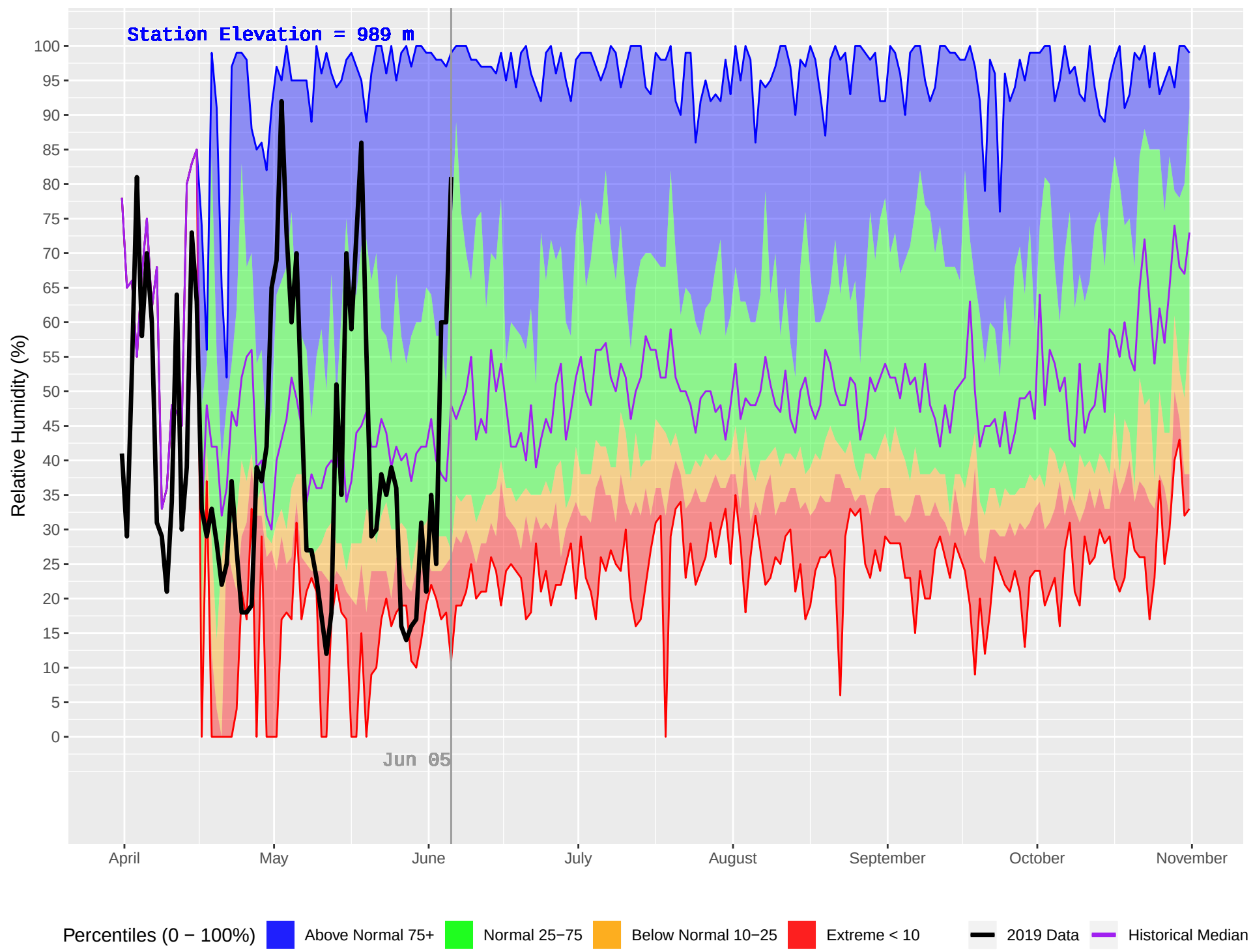
PINK MOUNTAIN (129) : Historical (1983–2018) and Current (2019) Daily Relative Humidity
