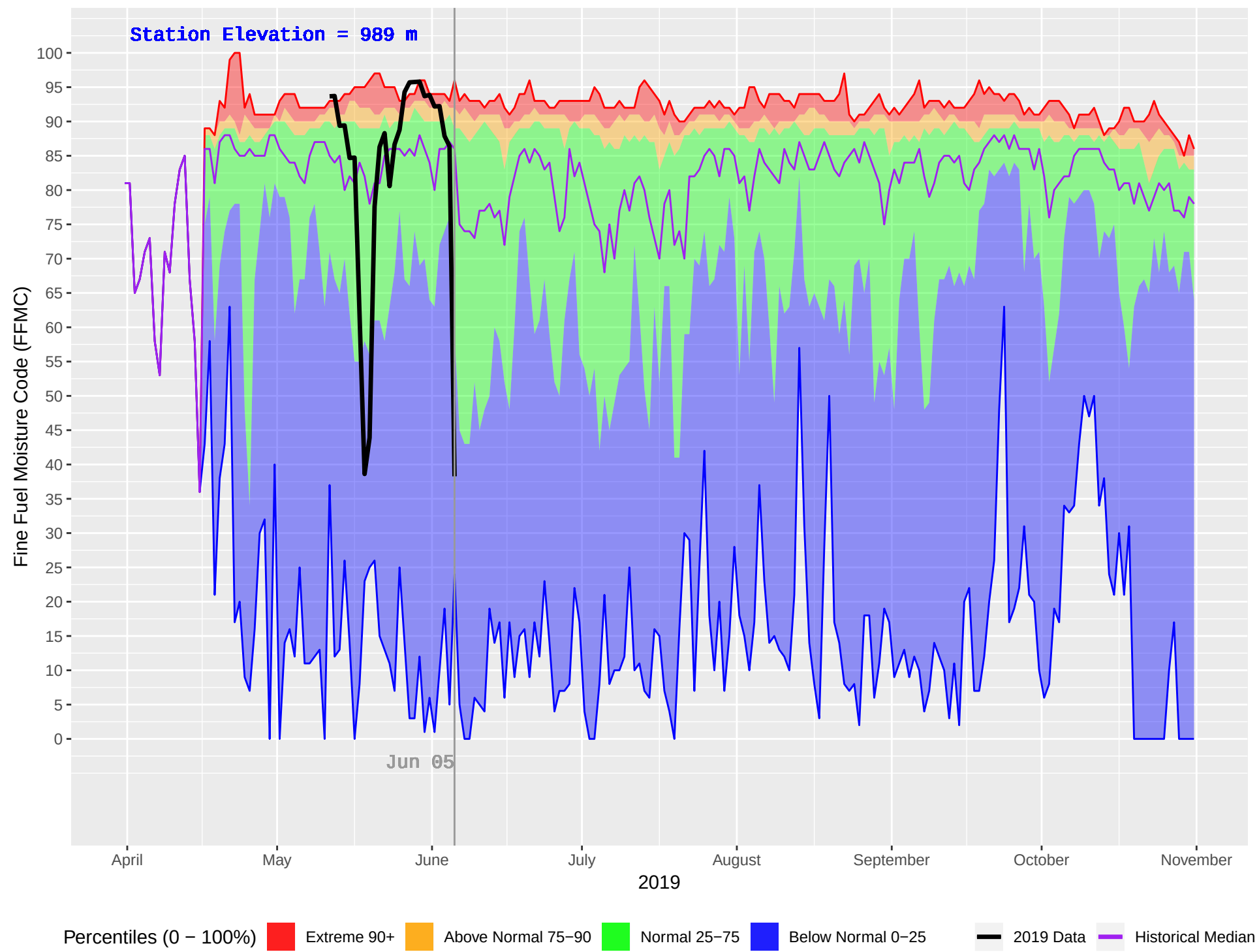
PINK MOUNTAIN (129) : Historical (1983–2018) and Current (2019) Daily Fine Fuel Moisture Code (FFMC)
