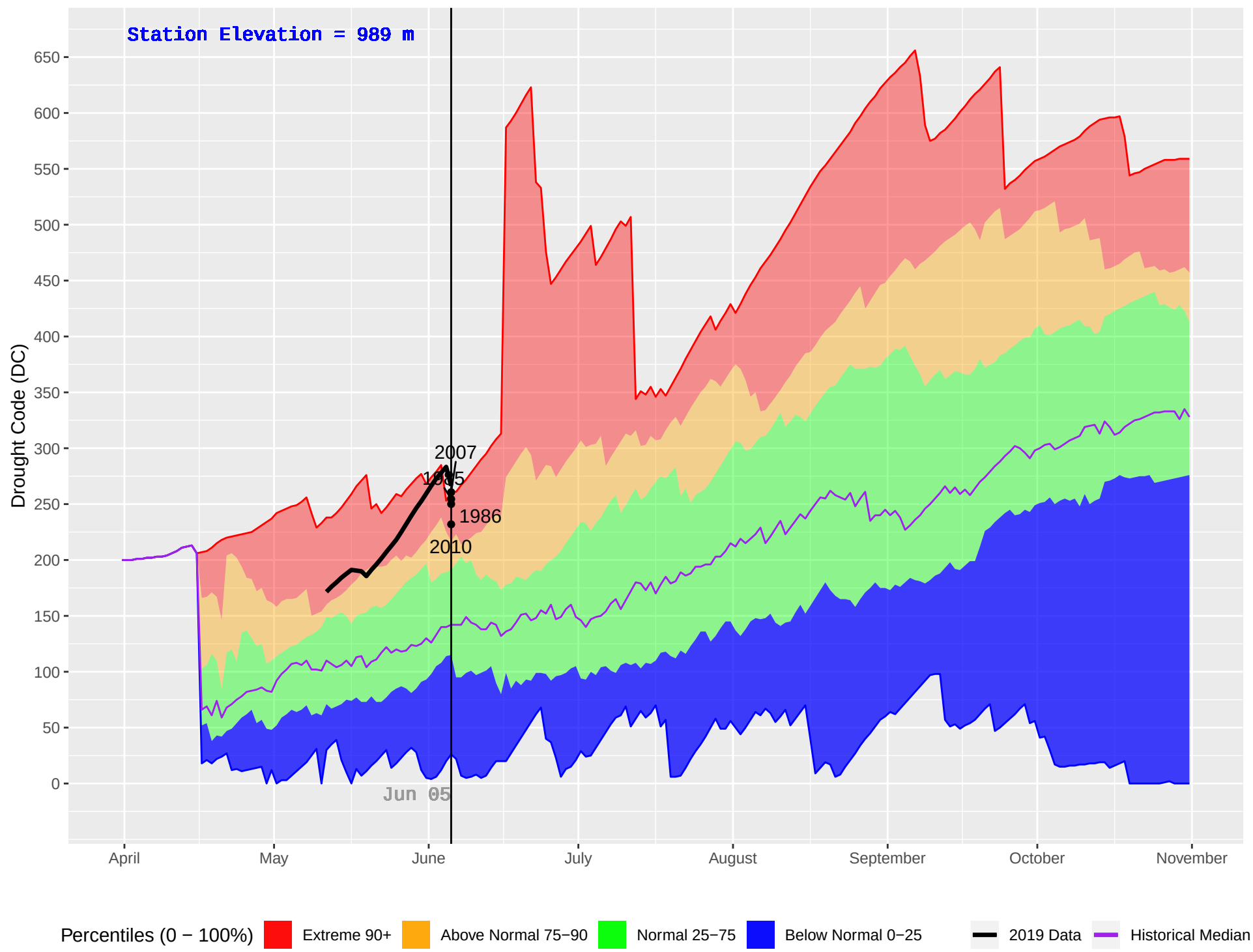
PINK MOUNTAIN (129) : Historical (1983–2018) and Current (2019) Daily Drought Code (DC)
