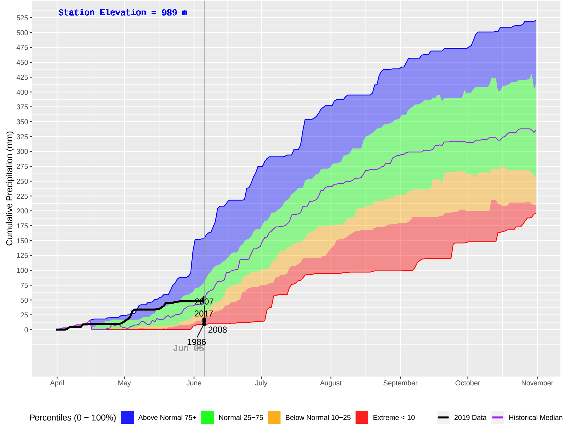
PINK MOUNTAIN (129) : Historical (1983–2018), Current (2019) Daily Cumulative Precipitation
