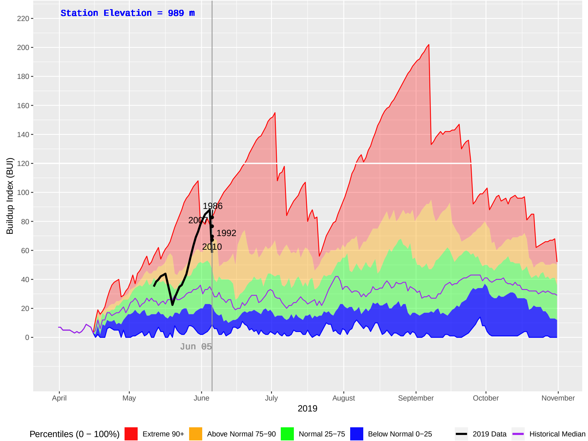
PINK MOUNTAIN (129) : Historical (1983–2018), Current (2019) Daily Buildup Index (BUI)
